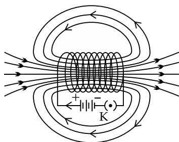
Field lines of the magnetic field through and around a current carrying solenoid 1
